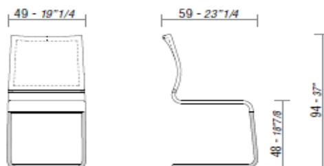
VERSO, chair in mesh on sled without armrests.
